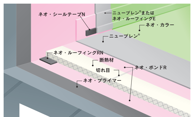
[NB-401工法]
